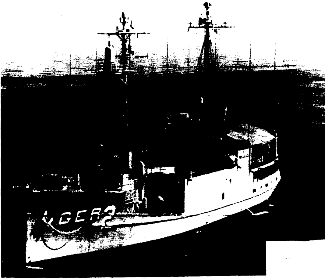
USS Pueblo shown following its conversion to AGER, December 1967.
