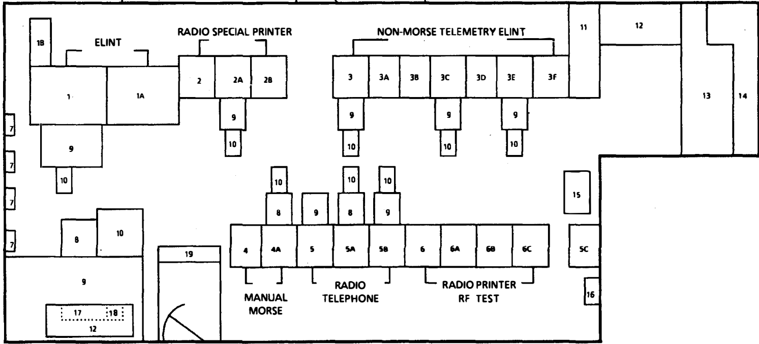
COMPARTMENT ARRANGEMENT AGER-2
